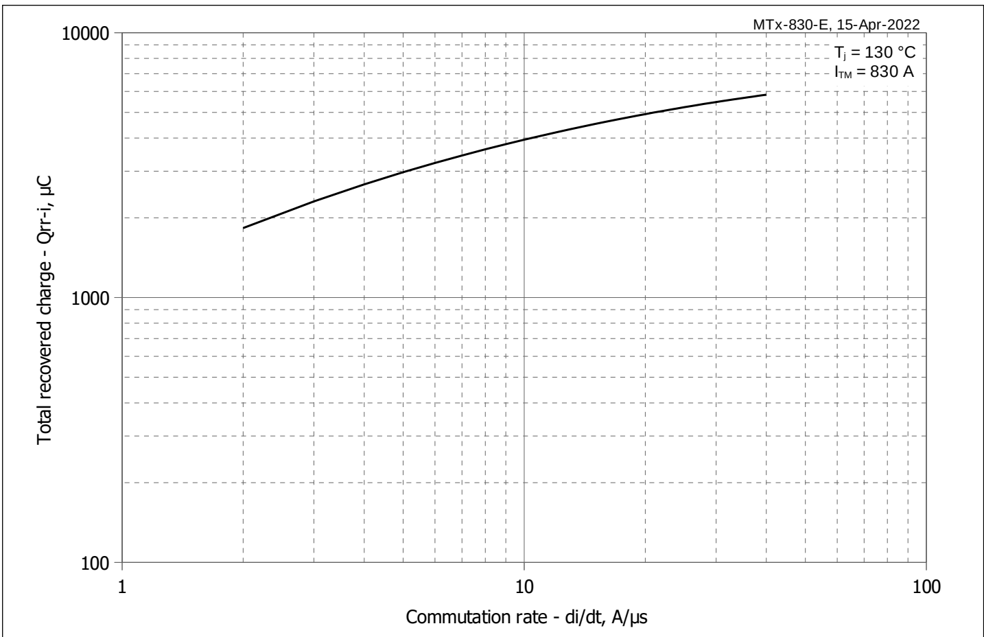
Fig 5 - Total recovered charge Q_{rr-i} (integral) vs. commutation rate di_R/dt
